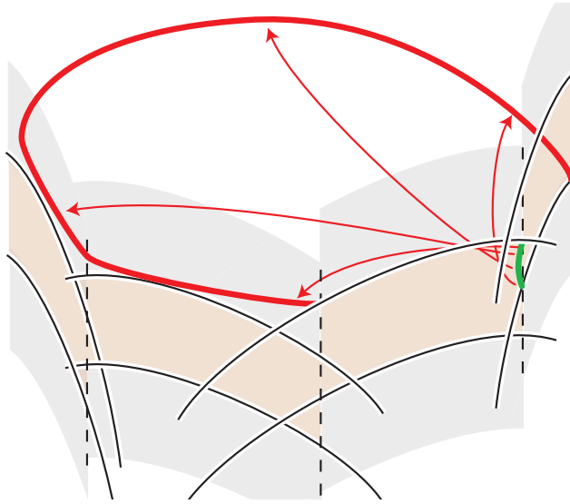
FIGURE 9. The effect of f_\gamma^\bullet on an arc that corresponds to a vertical side in the Ba'cfi-tiling.
