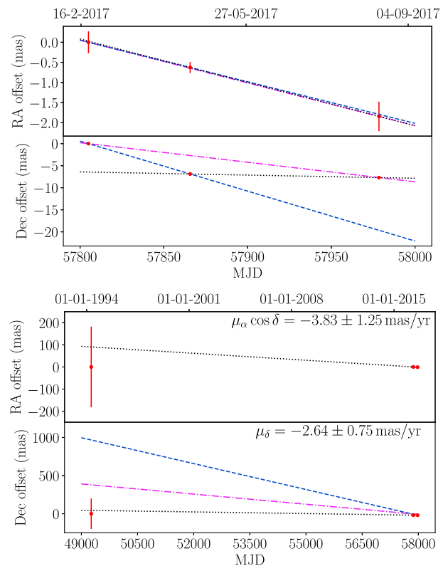
Figure 2. Proper motion fits for GRS 1716–249. GRS 1716–249 was tracked for three epochs over one outburst using the LBA, with positions shown with respect to the first LBA epoch. Top panel: fits by considering position measurements of two epochs at a time in RA and Dec. – epoch 1 and 2 (dashed line); epoch 2 and 3 (dotted line); epoch 1 and 3 (dot-dashed line). The three declination measurements do not lie on a straight line. Lower panel: fitting for proper motion by increasing the time baseline using the 1994 K -band image position measurement (dotted line), which breaks the degeneracy and shows that the epoch 1 LBA position is in error (blue and green dashed lines). This was then removed from the fit.
