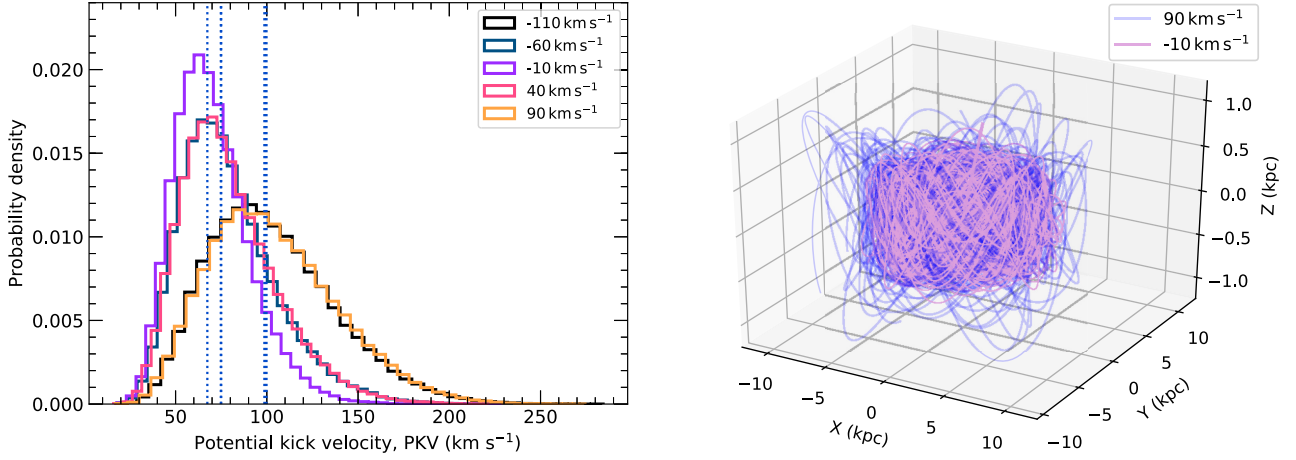
Figure 5. Left-hand panel: PKV probability distribution of GRS 1716–249 using Gaussian systemic radial velocity ( \bar{v} ) distributions with means of -110 , -60 , -10 , 40 , and 90 \text{ km s}^{-1} all with a 1\sigma of 50 \text{ km s}^{-1} . The medians of all the PKV distributions are the blue dashed vertical lines. The lowest PKV probability distribution median is of \sim 70 \text{ km s}^{-1} and corresponds to the systemic radial velocity of -10 \pm 50 \text{ km s}^{-1} . Right-hand panel: a 3D visualization of the Galactocentric orbit of GRS 1716–249, integrated for 1 Gyr for 20 orbit instances each of the lowest ( 67^{+41}_{-27} \text{ km s}^{-1} ) and highest ( 100^{+68}_{-47} \text{ km s}^{-1} ) PKV corresponding to systemic radial velocities of -10 \pm 50 and 90 \pm 50 \text{ km s}^{-1} , respectively. All three axes are in kpc. The system does not go beyond 1 kpc above the Galactic plane in both the cases.
