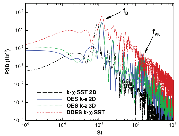
Fig. 11. Comparison of the power spectra density of the lift coefficients time-dependent evolution between URANS k - \omega SST, 2D and 3D OES- k - \varepsilon and DDES- k - \omega SST.
