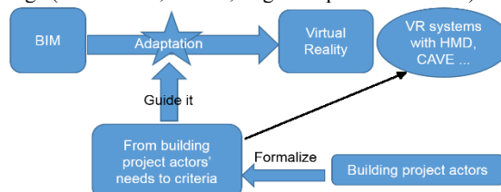
Figure 1: Methodology schema.
