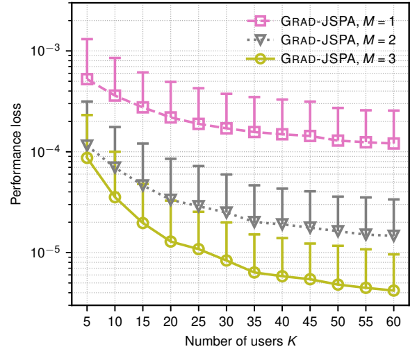
Fig. 4. Performance loss of GRAD-JSPA compared to the optimal WSR
