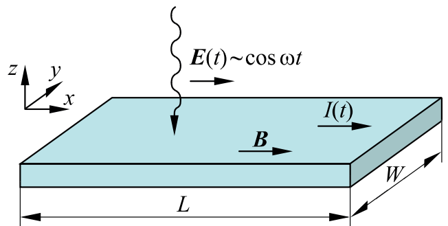
FIG. 1: A metal or semiconductor sample in a magnetic field \mathbf{B} and ac electric field \mathbf{E}(t) . The length of the sample, L , is much greater than its width, W . It is assumed that the ac electric field penetrates everywhere into the sample, i.e. that the electron system is either two-dimensional, or three-dimensional, but with thickness less than the skin depth.
