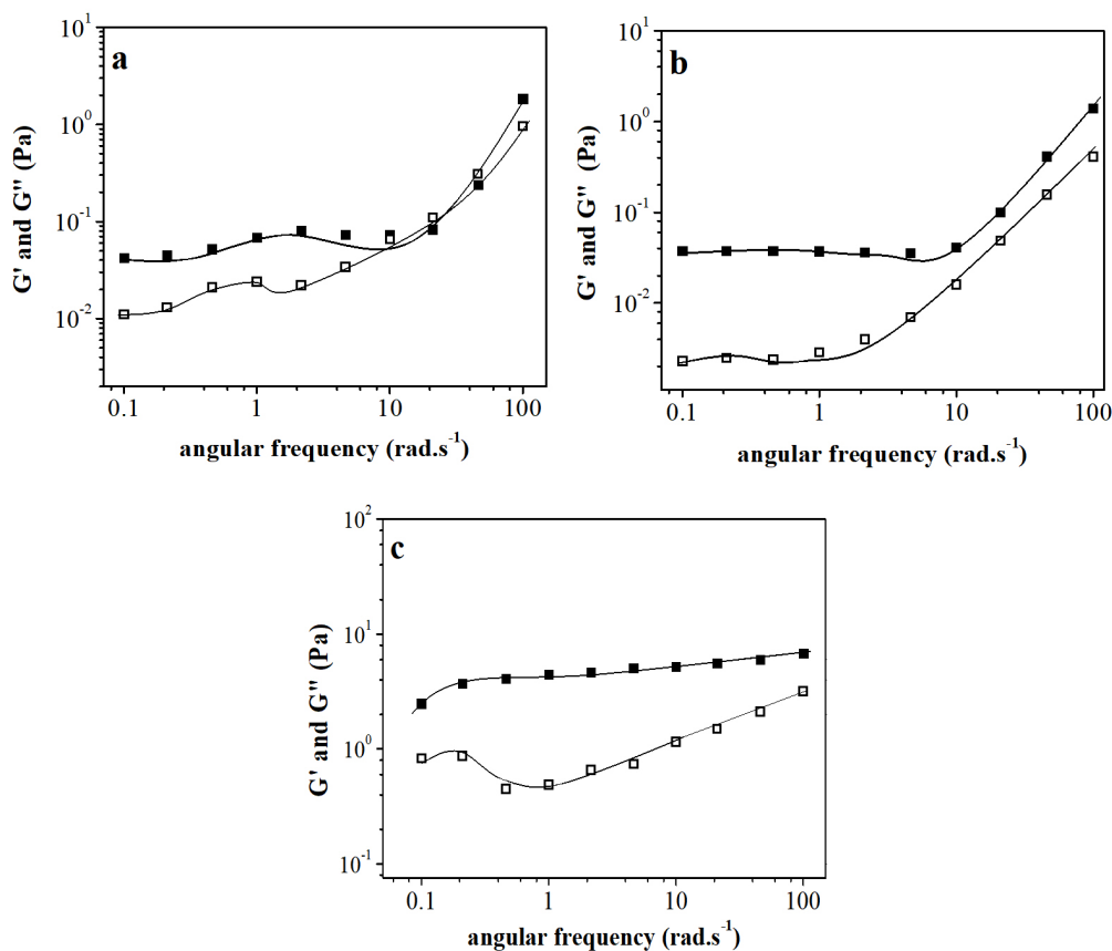
Figure 7. Storage, G' (solid symbols) and loss, G'' (empty symbols) moduli as a function of oscillation frequency for (a) CNC-t, (b) CNC-n and (c) CNF.
