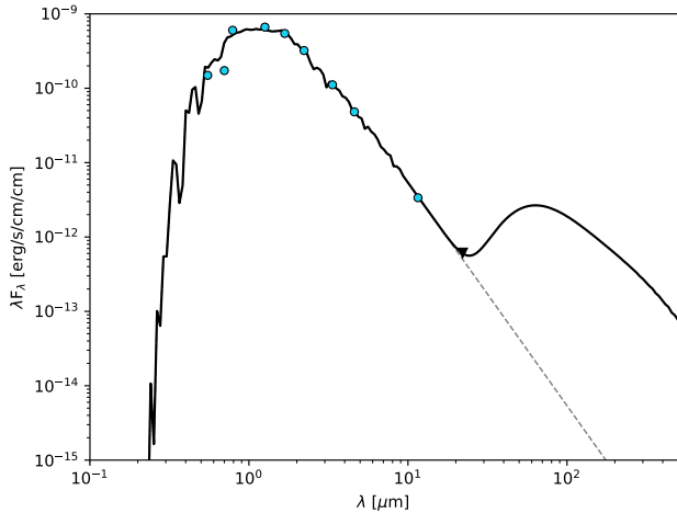
Fig. 6. SED of GSC 07396–00759, the photometry is shown in light blue, the stellar model in dashed gray, and the model with the maximum possible IR-excess compatible with observations is plotted in solid black.
