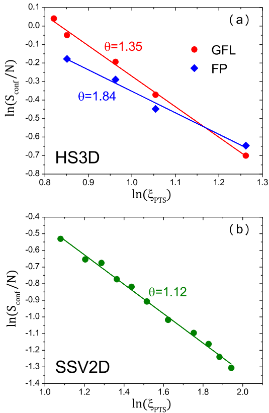
FIG. 4. S_{\text{conf}} vs. \xi_{\text{pts}} plot in d = 3 hard spheres (HS3D) (a) and d = 2 soft disks (SSV2D) (b). The straight lines are power law fits. For HS3D, we show two independent estimates of S_{\text{conf}} obtained from: the generalized Frenkel-Ladd (GFL) method and the Franz-Parisi (FP) free energy approach.
