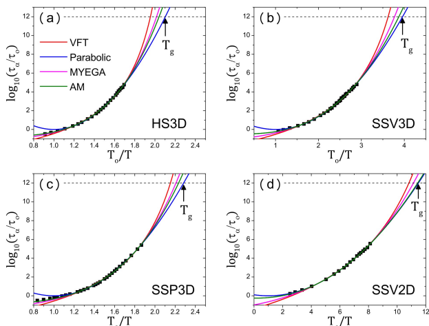
FIG. 2. Relaxation time as a function of inverse temperature for the four simulated models: HS3D (a), SSV3D (b), SSP3D (c), and SSV2D (d). The data are normalized by \tau_o and T_o , determined from a parabolic-law fitting. The horizontal dashed line indicates the timescale of the experimental glass transition, \tau_\alpha/\tau_o = 10^{12} . The vertical arrow indicates the experimental glass transition temperature T_g using the parabolic-law fitting. Three additional fitting functions are shown.
