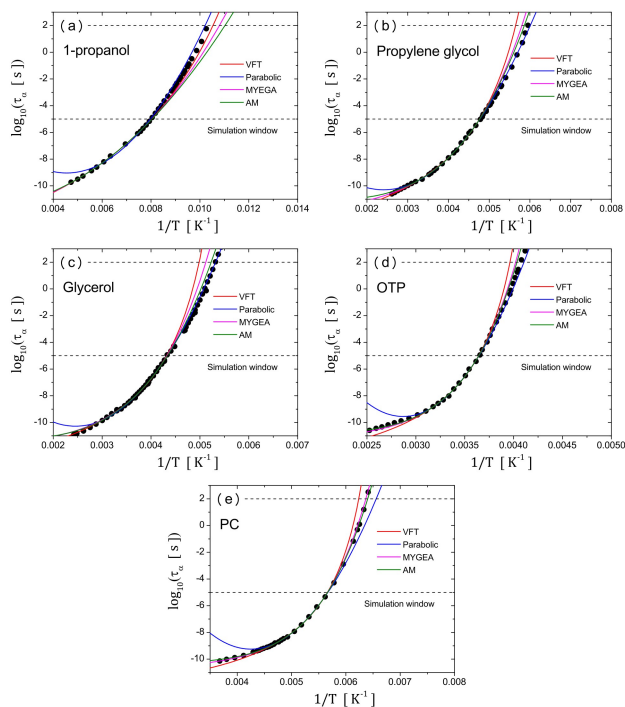
FIG. 8. Extrapolation from simulation timescale ( \tau_\alpha \leq 10^{-5} sec.) to experimental timescale for 1-propanol (a), propylene glycol (b), glycerol (c), OTP (d), and PC (e), whose kinetic fragility takes m = 35, 48, 53, 78, 104 , respectively. The values of m for 1-propanol, propylene glycol, and glycerol are comparable to the simulation models employed in this paper.
