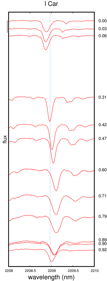
Fig. 2. Profile variations in the NaI 2208.969 nm line obtained from the CRILES spectra of I Car (the reference wavelength is indicated by the blue vertical dotted line). The black vertical line at the top left corresponds to a differential flux of 0.15. The pulsation phases are indicated to the right of each profile.
