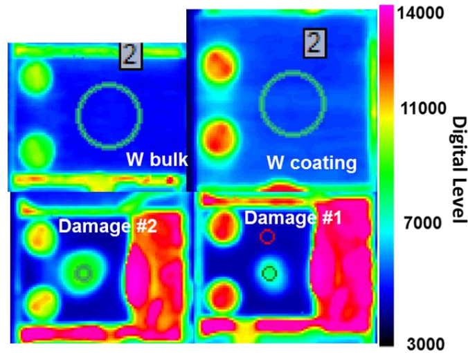
Figure 3. IR image illustration of the 4 samples at 250 °C and 3.9 μm: (top left) W bulk (top right) W coating (bottom left) W damaged samples with crack network and (bottom right) W damaged samples with cracks.
