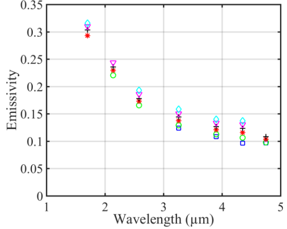
Figure 5. Emissivity of W bulk as function of the wavelength for several temperature: \square 300 ^{\circ}\text{C} , \circ 400 ^{\circ}\text{C} , * 500 ^{\circ}\text{C} , \diamond 600 ^{\circ}\text{C} , \blacktriangledown 700 ^{\circ}\text{C} , + 800 ^{\circ}\text{C} .
