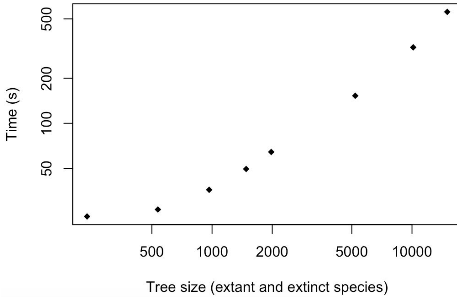
Figure S2. Computing time for different simulation in a computer with a 3,4 GHz Intel Core i5 processor. The rates used were Duplication rate: 0.2, Transfer rate: 0.2, Loss rate: 0.6, Origination rate:0.05, Inversion rate: 0.2, Translocation rate: 0.2. The initial genome was composed of 500 genes. All extension rates were set to 1. Species trees were obtained using by setting Speciation rate: 1 and Extinction rate: 0.5.
