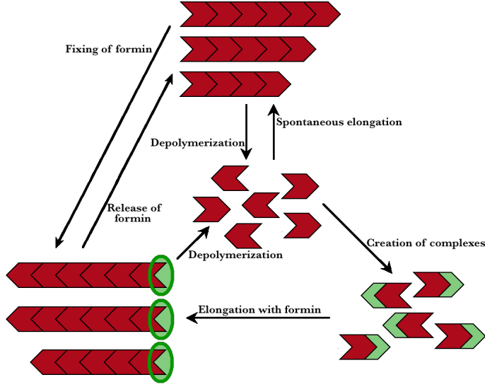
Fig. 2: Transitions in the model for a population of polymers. Simple polymers can elongate by catching a free monomer, release a monomer that becomes free, or switch to the “fast” mode by binding with a formin. Polymers bound with a formin can elongate by catching a G-actin/profilin complex, release a monomer that becomes free, or switch to the “normal” mode by releasing the attached formin. Finally, free monomers and profilins can bind to form G-actin/profilin complexes.
