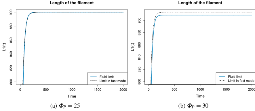
Fig. 4: Evolution of the length of the filament with N = 1000 , \lambda^+ = 10 , \lambda^- = 2 , \lambda_F^+ = 100 , \Phi_F^+ = 1 and \Phi_F^- = 1 for two values of \Phi_P . Initially, there are a (unique) polymer of length 334, 333 free monomers and 333 G-actin/profilin complexes. On each graph, we plot the fluid limit given in Theorem 11 ( i.e. , N times l_i(t) ) and the fluid limit assuming that the system stays in fast mode all the time.
