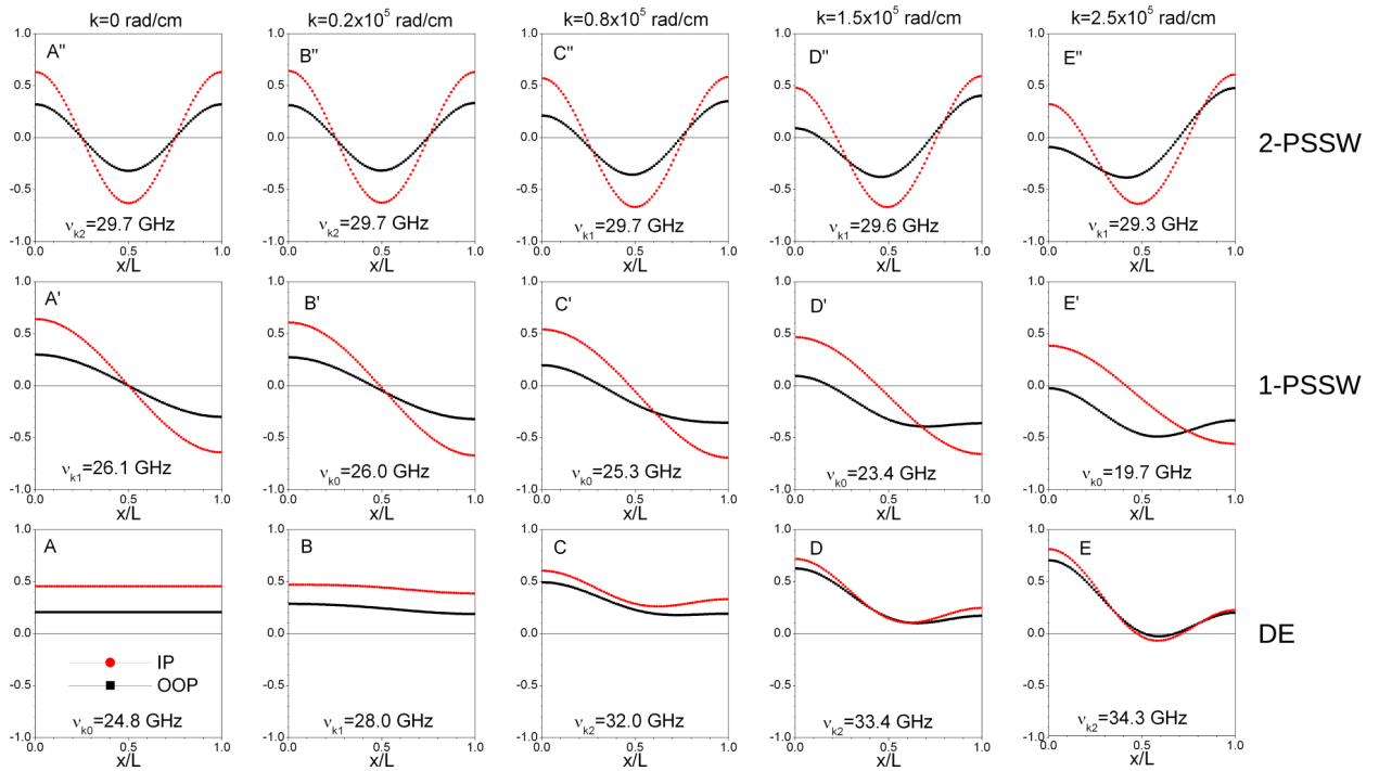
FIG. 5. The distribution of the two dynamic magnetization components, namely the out-of-plane one m_k^y(x) (OOP, black line) and the in-plane one m_k^x(x) (IP, red line), across the film thickness ( 0 < x/L < 1 ), for the various points denoted by capital letters (A, A', A''), (B, B', B''), etc. in the dispersion curves of Fig. 4. The intensity of the in-plane applied magnetic field is H = 4 kOe.
