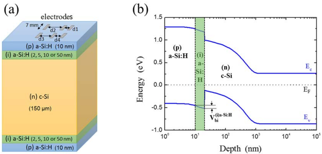
Figure 1. (a) Sketch of the solar cell studied here. The various inter-electrode distances are d_1=1.8 mm, d_2=6.5 mm, d_3=5 mm, d_4=3.15 mm. (b) Equilibrium band diagram of the structure calculated with 10 nm of (i) a-Si:H ( E_c : conduction band energy, E_v : valence band and E_F : Fermi level). V_{bi}^{(i)a-Si:H} is the potential drop in the (i) a-Si:H layer. Note the logarithmic scale for the depth, referred to the top surface.
