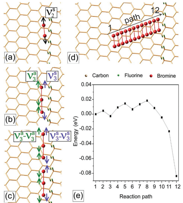
Fig. 2 Fragments of fluorinated graphene with adsorbed Br_2 (a), Br_3 (b) and Br_6 (c) species. Arrows indicate the directions of atomic motion for normal stretching modes of Br_2 ( \nu_2^s ), Br_3 ( \nu_3^a and \nu_3^s ), and Br_6 ( \nu_3^a-\nu_3^a and \nu_3^s-\nu_3^s ). Diffusion path of Br_2 over partially fluorinated graphene layer from the non-fluorinated area (position 1) to the fluorine chain (position 12) (d). NEB path was constructed automatically from position 1 to 12. Diffusion barrier of Br_2 over partially fluorinated graphene (e).
