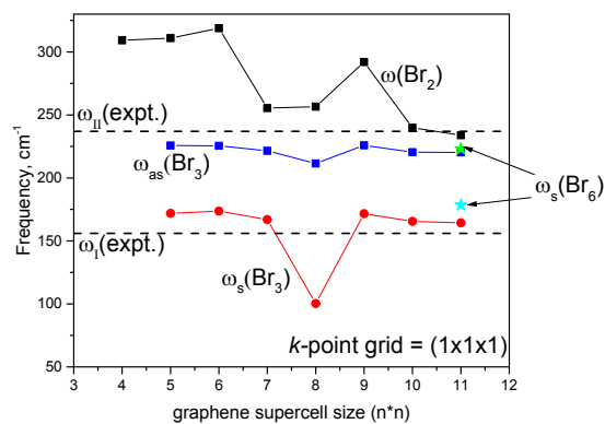
Fig. S2 Variation in calculated charge (a) and stretching frequencies (b) of Br 2 , Br 3 and Br 6 located over graphene sheet with the size of graphene supercell and k-point grid. Dashed lines in (b) correspond to peak I and II of experimental Raman spectra of brominated graphite and bromine-intercalated fluorinated graphites (see Fig. 1).
