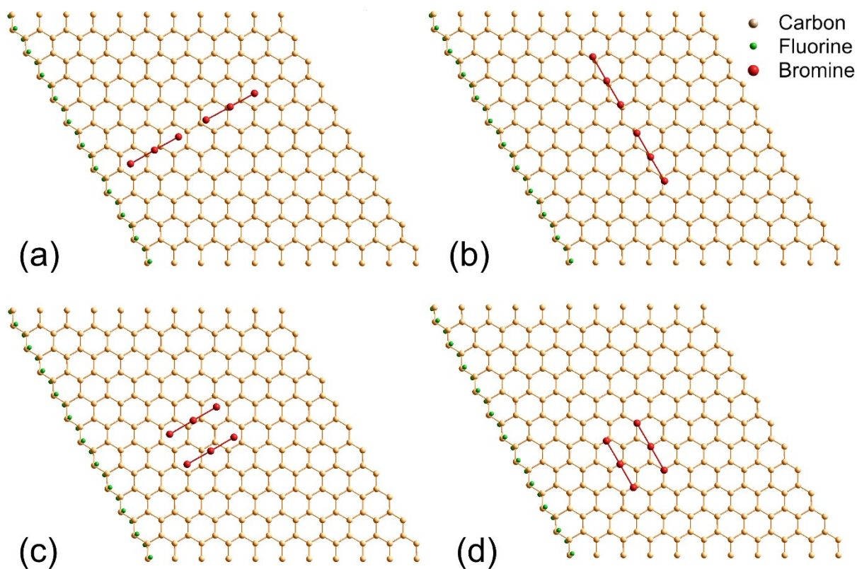
Fig. S3 Optimized geometries of metastable structures of Br 6 over partially fluorinated graphene sheet.
