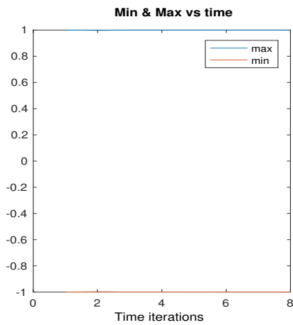
Figure 12: Cameraman image. On lines 1 and 2: from original image to its segmentation (with RSS scheme) \Delta t = 5.e - 7 , \epsilon = 0.04 , \tau = 1 , \lambda = 10^{10} . On line 3: min and max values vs time iterations (left) and L^2 norm of the discrete time derivative of the solution vs time iterations.
