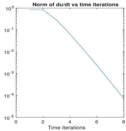
Figure 12: Cameraman image. On lines 1 and 2: from original image to its segmentation (with RSS scheme) \Delta t = 5.e - 7 , \epsilon = 0.04 , \tau = 1 , \lambda = 10^{10} . On line 3: min and max values vs time iterations (left) and L^2 norm of the discrete time derivative of the solution vs time iterations.
