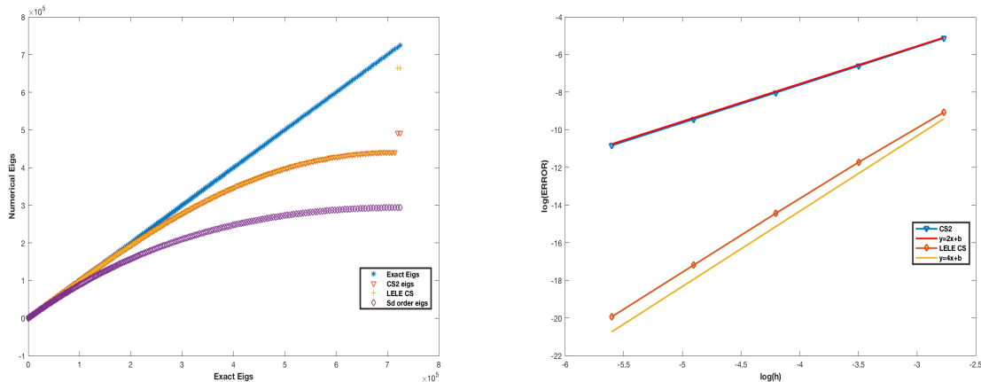
Figure 1: Spectrum of the laplacian matrix discretized with second order and fourth order compact schemes (Lele’s and CS2) compared to the exact spectrum of the operator (left); L^\infty error to the function u(x) = \cos(x(1 - x)) when varying the step-size h , for the 3 schemes - comparison with lines of slope 2 and 4.
