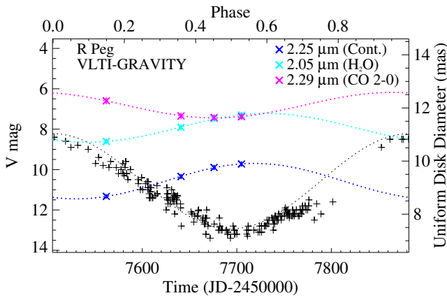
Fig. 1. Variability in the V magnitude and in the UD angular diameters in the near-continuum band, and in bands dominated by \text{H}_2\text{O} ( 2.05 \mu\text{m} ) and \text{CO} 2–0 ( 2.29 \mu\text{m} ). Also shown are sinusoidal fit results. The minimum continuum size tracks the maximum light, which can be understood by the increasing effective temperature when the star gets smaller. The minimum contribution of \text{H}_2\text{O} tracks the maximum light as well, which can be understood as the destruction of water vapour at maximum light and formation at minimum light. The contribution from \text{CO} instead is greatest at maximum light, indicating a different and more stable behaviour of \text{CO} compared to water vapour.
