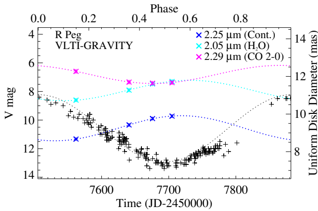
Fig. 1. Variability in the V magnitude and in the UD angular diameters in the near-continuum band, and in bands dominated by \text{H}_2\text{O} ( 2.05\ \mu\text{m} ) and CO 2–0 ( 2.29\ \mu\text{m} ). Also shown are sinusoidal fit results. The minimum continuum size tracks the maximum light, which can be understood by the increasing effective temperature when the star gets smaller. The minimum contribution of \text{H}_2\text{O} tracks the maximum light as well, which can be understood as the destruction of water vapour at maximum light and formation at minimum light. The contribution from CO instead is greatest at maximum light, indicating a different and more stable behaviour of CO compared to water vapour.
