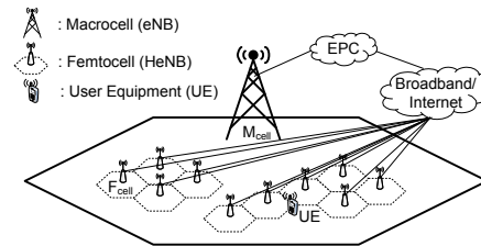
Figure 1. LTE femtocell/macrocell network architecture.
