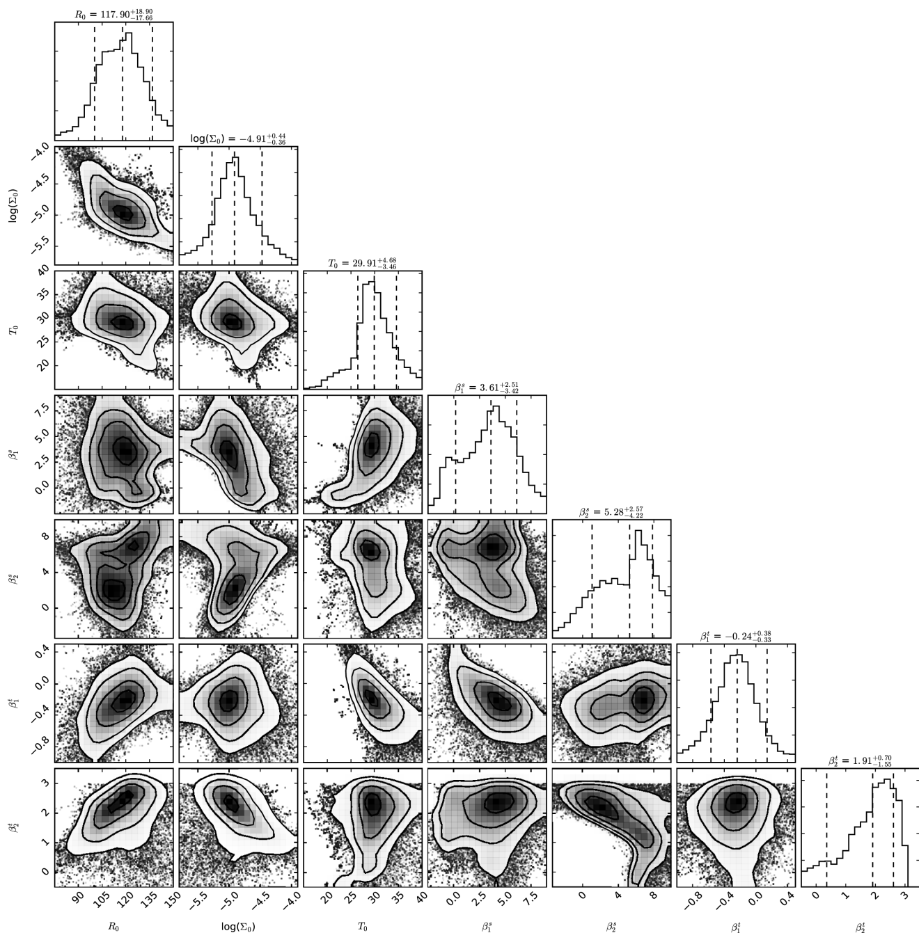
Figure 14. Posterior distribution of the double power-law gas model for R_0 , \Sigma_0 , T_0 , \beta_1^s , \beta_2^s , \beta_1^t , \beta_2^t (see Section 4.2.2). The marginalized distributions are presented in the diagonal. The vertical dashed lines represent the 16th, 50th, and 84th percentiles.
