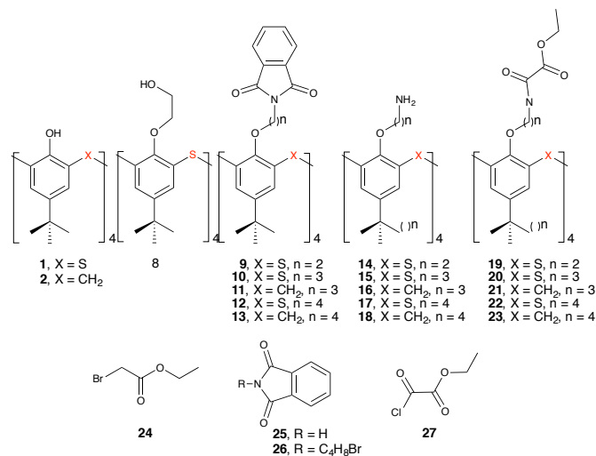
Figure 2: Starting compounds 1 and 2 , precursors 8-27 used for the synthesis of ligands 3-7 .
