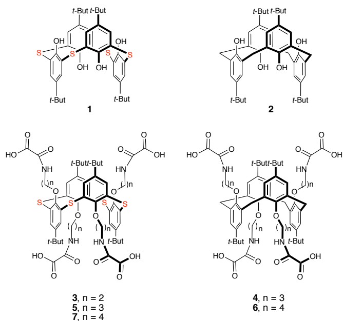
Figure 1: p - tert -butylthiacalix[4]arene TCA 1 and p - tert -butylcalix[4]arene CA 2 in 1,3 -Alternate conformation and their derivatives bearing four oxamate units 3-7 .
