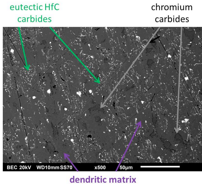
Figure 3: As-cast microstructure of the FeHfC alloy (SEM/BSE micrograph).
