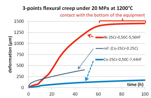
Figure 6: The obtained deformation curves (except the one of FeHfC which was too fast and stopped much sooner than 100h); comparison with the one previously obtained for a ternary cobalt-base alloy).
