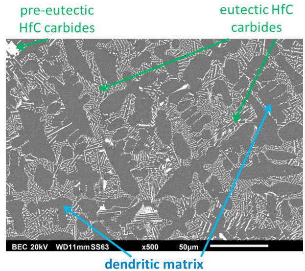
Figure 1: As-cast microstructure of the CoHfC alloy (SEM/BSE micrograph).
