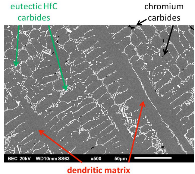
Figure 2: As-cast microstructure of the NiHfC alloy (SEM/BSE micrograph).
