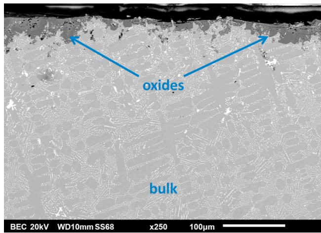
Figure 7: Sub-surface of the CoHfC alloy after 50h of oxidation in air at 1200°C.
