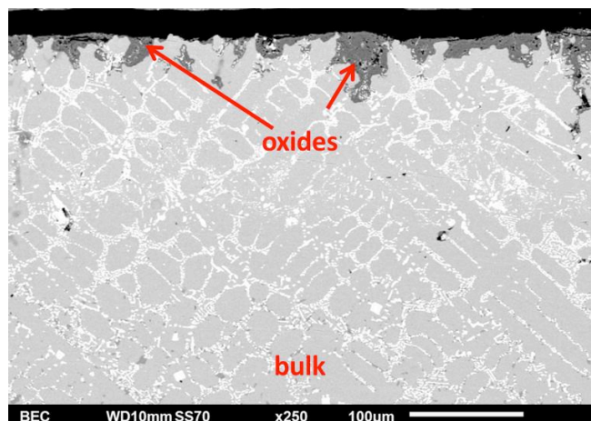
Figure 8: Sub-surface of the NiHfC alloy after 50h of oxidation in air at 1200°C.
