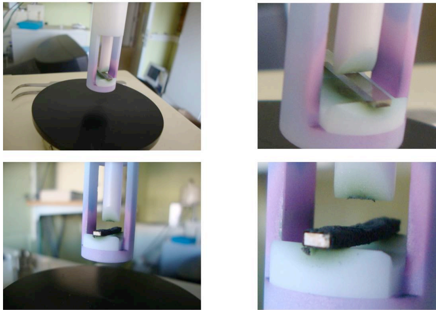
Figure 4: Photographs of the apparatus used for the bending creep tests; sample before test (top) and sample after test (bottom).
