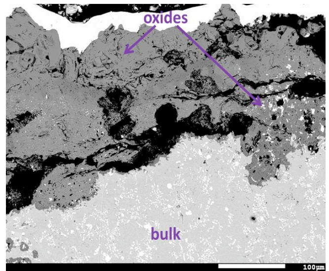
Figure 9: Sub-surface of the FeHfC alloy after 50h of oxidation in air at 1200°C.
