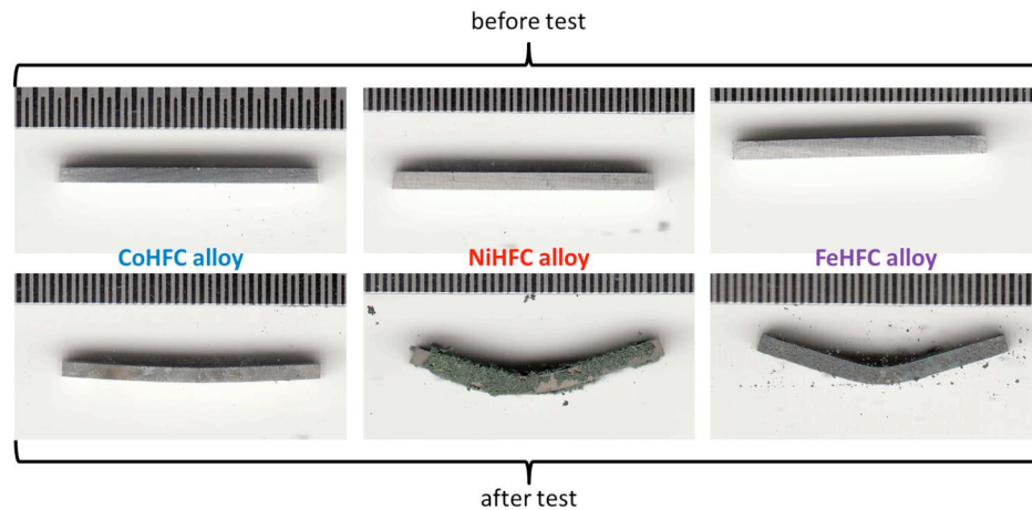
Figure 5: Photographs of the three samples before test (top) and sample after test (bottom).
