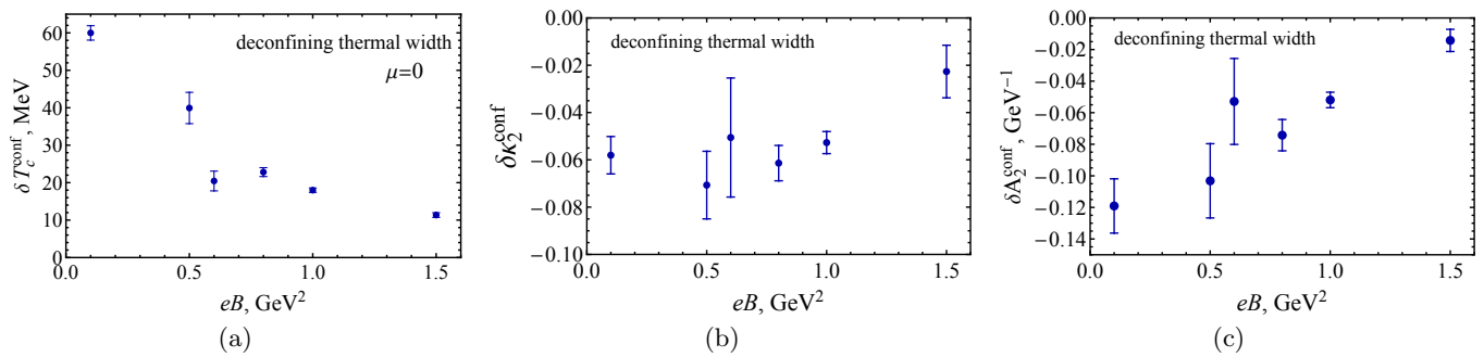
FIG. 13. (a) The thermal width \delta T_c of the deconfining crossover at zero chemical potential \mu_B = 0 , as well as the curvature of the deconfining thermal width in (b) the dimensionless units \delta \kappa_2 , and (c) physical units \delta A_2 vs. the magnetic-field strength B .
