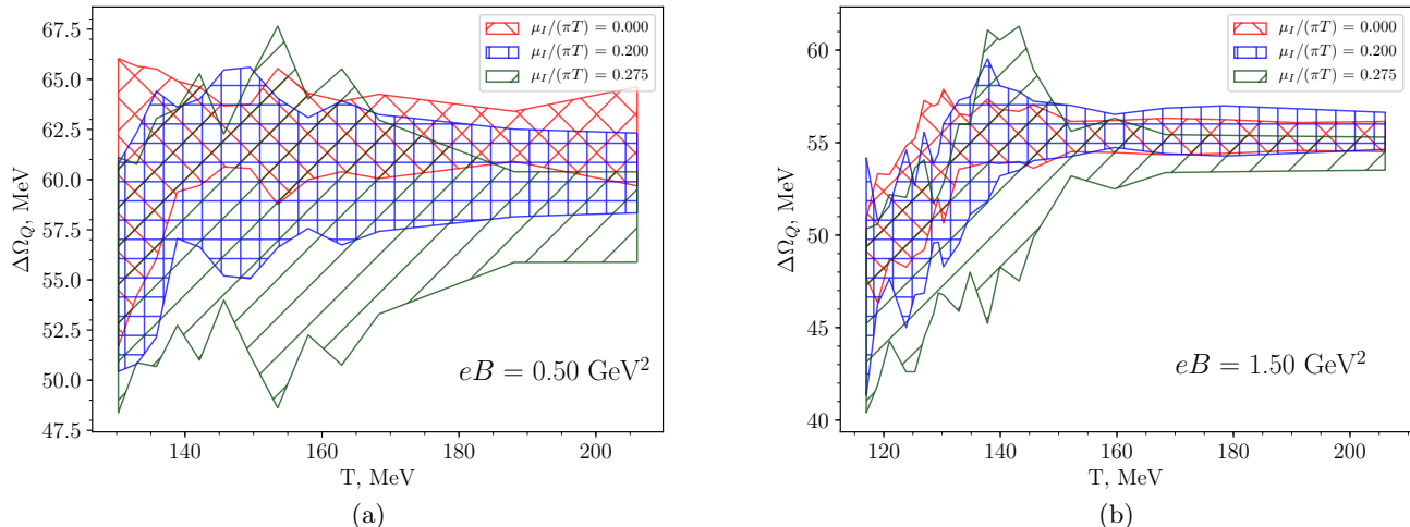
FIG. 17. The difference between free energies (A4) at the renormalization scales \tilde{f} = 0.54 fm and f = 0.80 fm, for the magnetic field strengths (a) eB = 0.5\text{GeV}^2 and (b) eB = 1.5\text{GeV}^2 . Three different values of the imaginary chemical potential \mu_I are represented by different colors.
