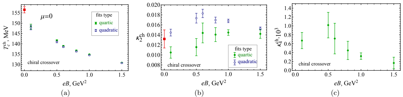
FIG. 5. (a) The critical temperature T_c^{\text{ch}} of the chiral crossover at \mu_B = 0 , as well as the curvatures (b) \kappa_2 and (c) \kappa_4 as functions of the magnetic-field strength B . The first two quantities are obtained with the help of both quadratic and quartic versions of the fitting function (18), with fits shown in Fig. 4. The red points in plots (a) and (b) correspond to the known results at B = 0 . They are taken from Refs. [4] and [9], respectively.
