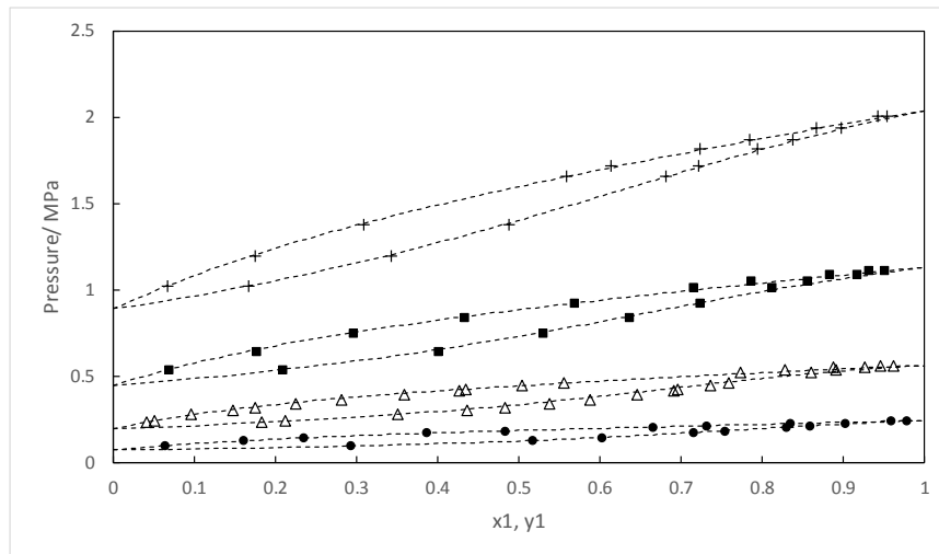
Fig. 1: Pressure as a function of n-butane mole fraction in the n-butane (1) + Ethylmercaptan (2) mixture at different temperatures. ●: 298.14 K, Δ : 328.04 K, ■: 358.11 K, +: 388.18 K. Dashed lines: calculated with PR EoS with binary interaction parameters from Table 4.
