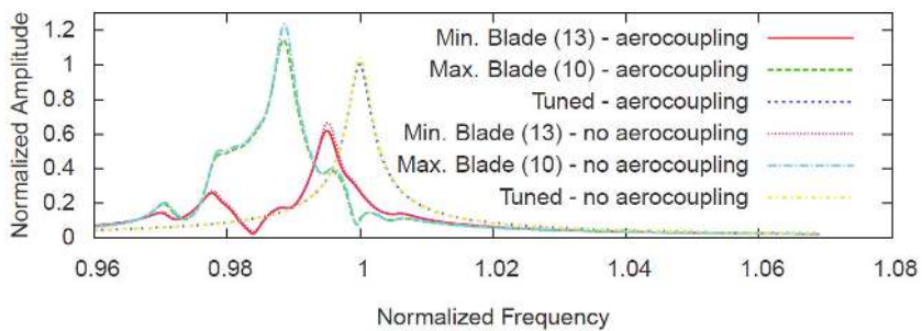
Figure 3. Frequency response function for tuned and mistuned bladed disks with aeromechanical coupling
