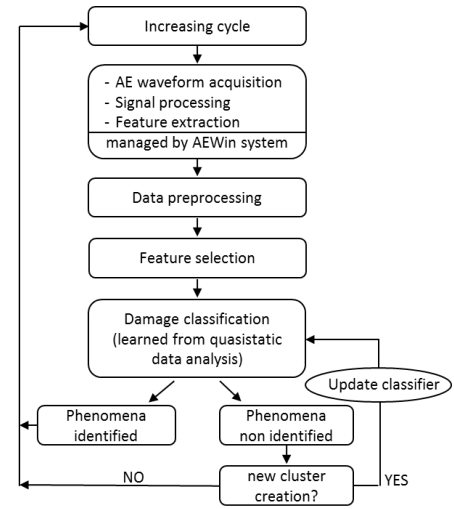
Figure 1. Unsupervised damage detection methodology
