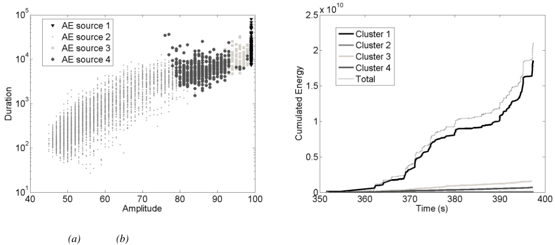
Figure 10. Learning phase: (a) AE data segmentation represented by Duration vs. Amplitude ; (b) Evolution of AE cumulated energy of each AE source
