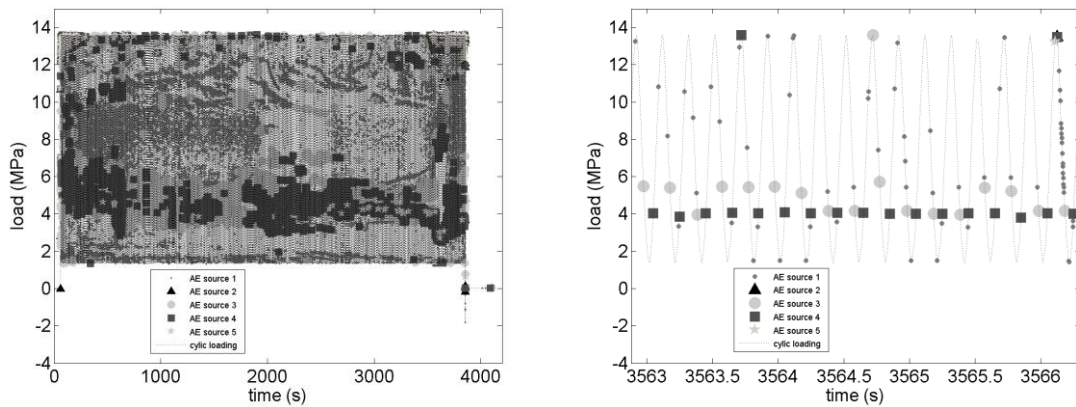
Figure 13. Classified AE events during cyclic loading: (a) global visualization (b) zoomed view of some cycles
