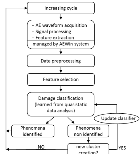
Figure 1. Unsupervised damage detection methodology
