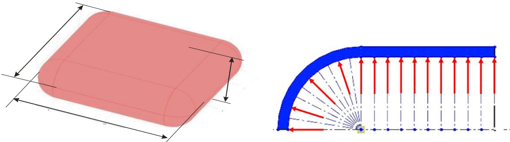
Figure 2. Example of a form fitted improvement – Pressure field on a cross section
