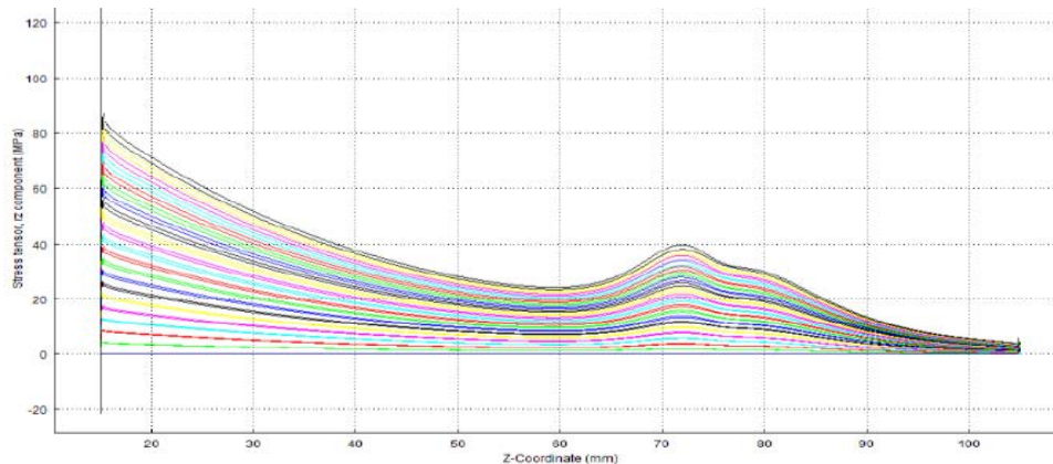
Figure 5. Numerical study of the shear stress in the adhesive joint – Cone angle 5°
