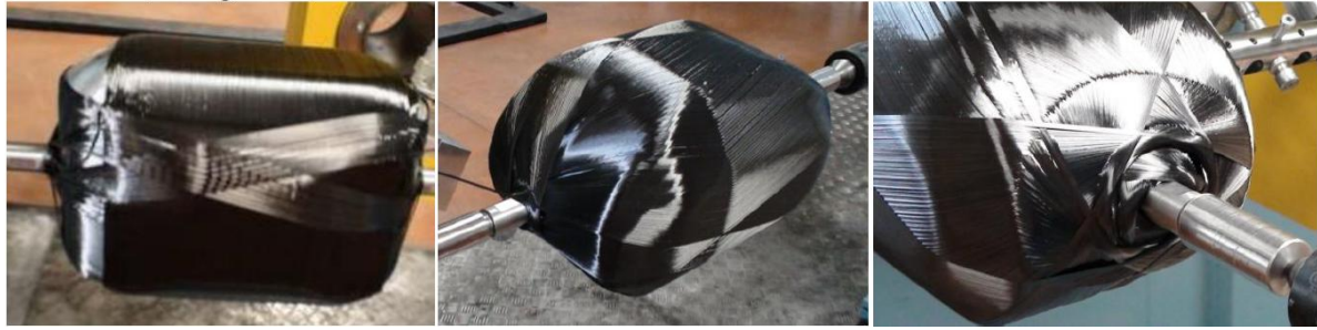
Figure 9. Filament winding of the form-fitted tank
