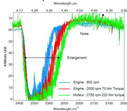
Fig. 2 : Typical gas absorption lines for carbon dioxide in the infrared.
