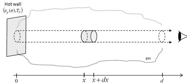
Fig. 3 : Typical experimental configuration.
