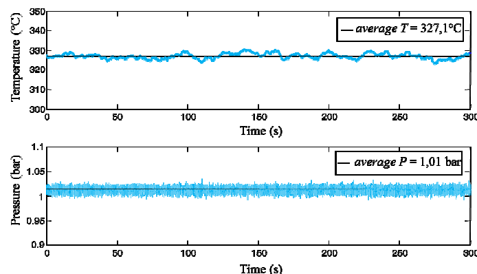
Fig. 7 : Temperature and pressure for a 5%CO 2 and 95%N 2 mixture
