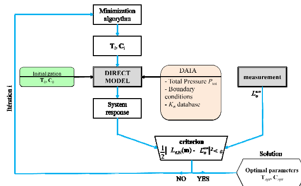
Fig. 5 : Principle of the optimization code.
