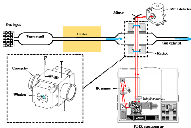
Fig. 6 : Experiment setup on synthetic gas bench for measurement of the transmission spectrum.
