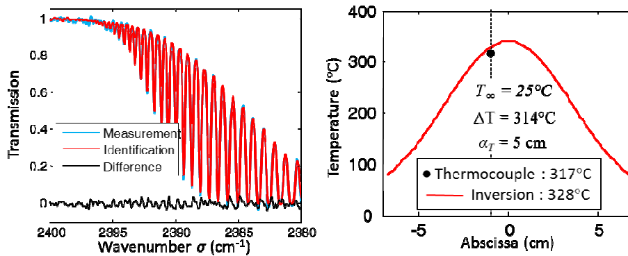
Fig. 9 : Inversion results on the transmission measurement for a DV6-TED4 car engine at 2500rpm and 40Nm torque
