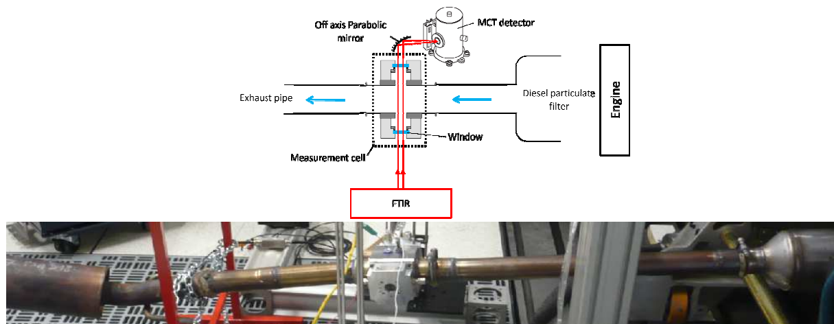
Fig. 8 : Instrumentation set-up for radiative measurement of exhaust gas for a DV6-TED4 Diesel engine
