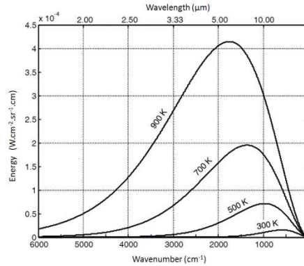
Fig. 1 : Energy emitted by a black body for various temperatures
