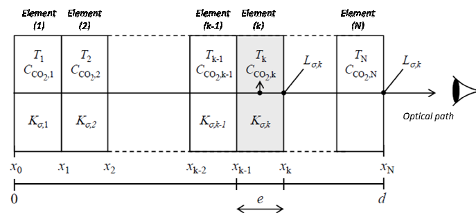
Fig. 4 : Heterogeneous system divided into N homogeneous and isotherm elements.
