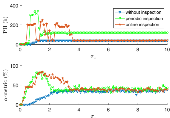
Fig. 15. Prognostic performances with different \sigma_\omega .
