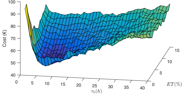
Fig. 9. Estimation cost surface for online triggered covariate inspection J(ET, \tau_h)
