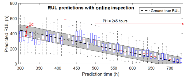
Fig. 14. RUL predictions with online inspections.
