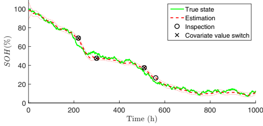
Fig. 10. Estimation with online triggered inspection
