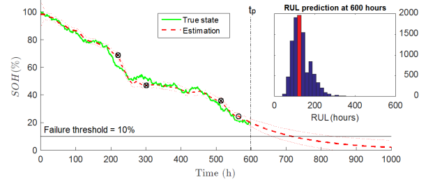
Fig. 13. Degradation estimation with online inspections and RUL prediction at t_p = 600 hours.
