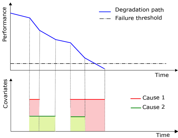
Fig. 1. Degradation path and covariates.
