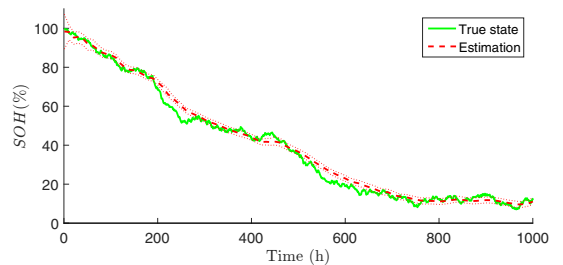
Fig. 3. Estimation without inspection.
