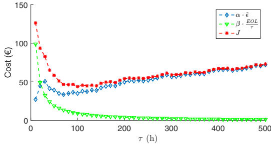
Fig. 5. Cost curve for estimation with periodic inspection.
