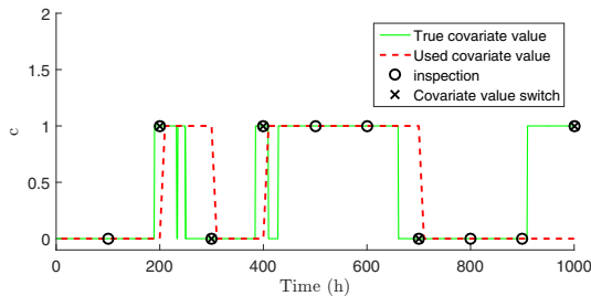
Fig. 7. Periodic inspection for covariates.
