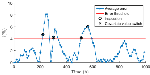
Fig. 12. Estimation error with online triggered covariate inspection.
