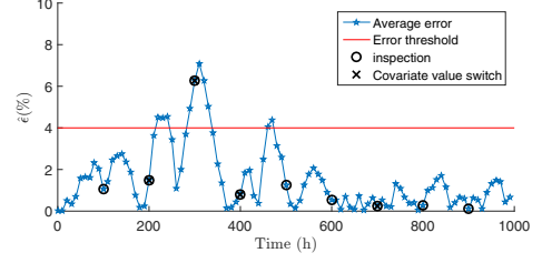
Fig. 8. Estimation error with periodic inspection.
