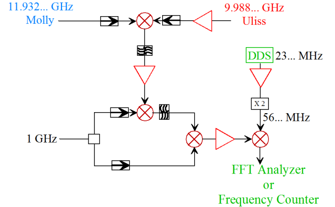
Fig. 3. Measurement system for phase noise and stability characterization of the microwave outputs of the two CSOs.
