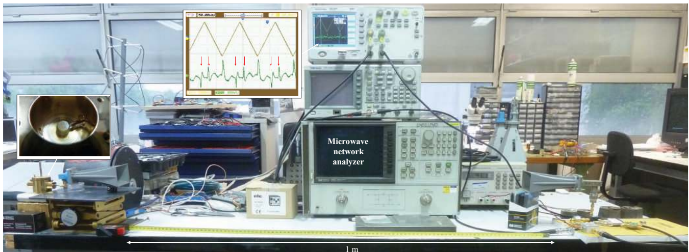
FIG. 6. Experimental setup demonstrating the interrogation range of over 1 m.
