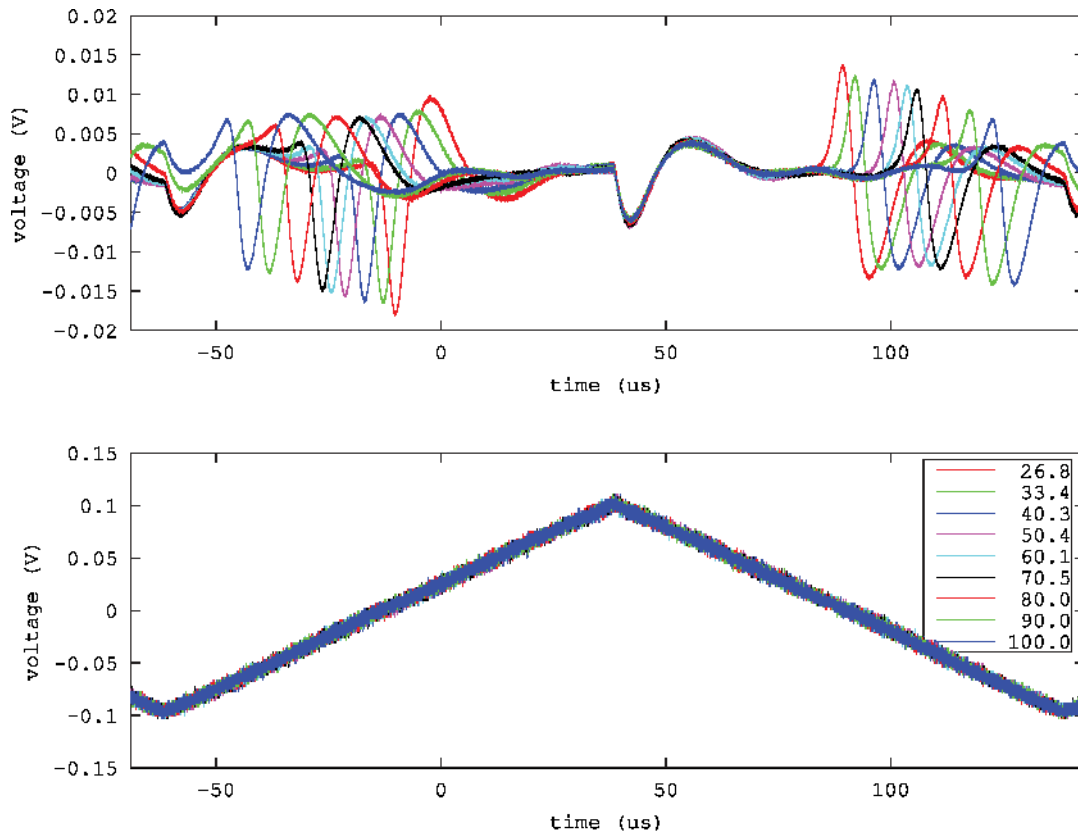
FIG. 3. Bottom: triangle shaped signal driving the VCO. The legend indicates the temperature at which each curve is recorded (in °C). Top: signal returned from the dielectric resonator as a function of temperature. The legend indicating the dielectric resonator temperature at which each curve was collected is valid for both graphs.
