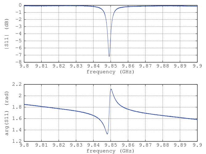
FIG. 1. Dielectric resonator reflection coefficient characterization (top: magnitude, bottom: phase).
