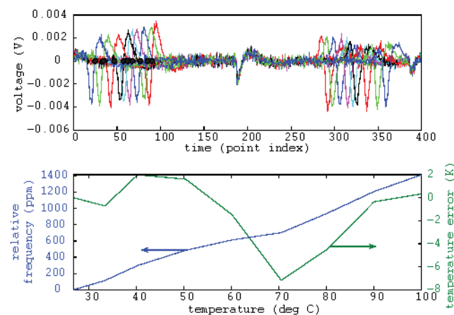
FIG. 4. Derivate of the returned signal for a precise identification of the resonance frequency. Top: the time axis is provided in sample index to account for the oversampling when estimating the zero-crossing condition of the signal derivate (linear interpolation: the black circles indicate the zero crossing abscissa). Bottom: extracted temperature dependence of the dielectric resonator (left axis) with a first order coefficient resulting from a linear fit of the relative frequency dependence with temperature, and resulting measurement error (right axis) resulting from the subtraction of the estimated temperature and the measured outer resonator cavity temperature—the standard deviation of the measurement error (right axis) is 3 K.
