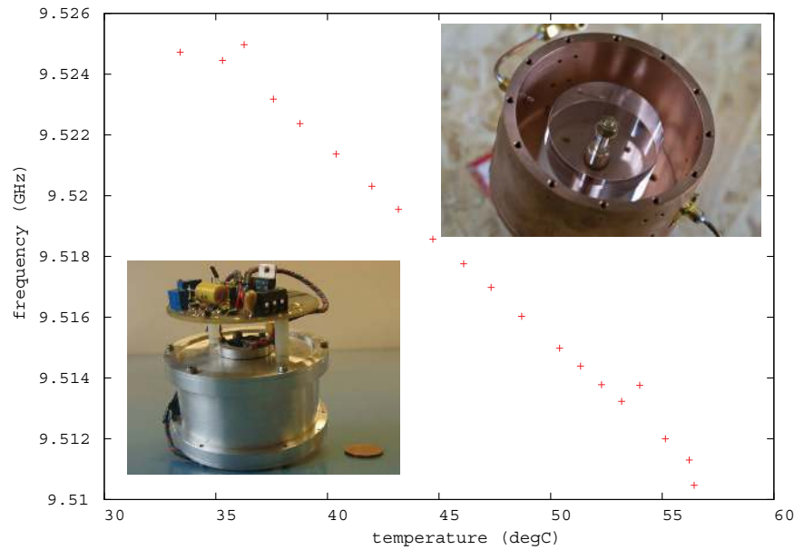
FIG. 5. Wireless characterization of a sapphire resonator resonance frequency temperature dependence, probed on the \text{WGH}_{8,0,0} whispering gallery mode. Insets: pictures of the cavity containing the sapphire resonator (top right) and circuit for controlling the resonator temperature (bottom left).
