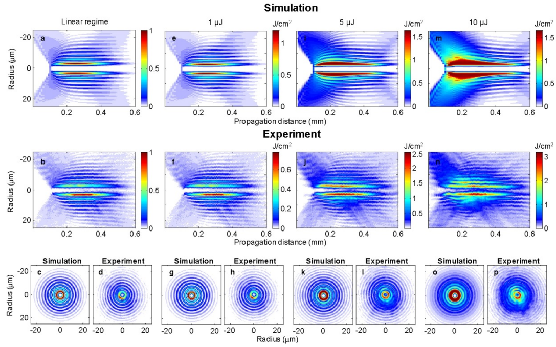
Figure 3. Stationary regime of Nonlinear Bessel Vortices. The fluence distribution, in \text{J} \cdot \text{cm}^{-2} , is recorded for different input pulse energies. The cone angle is 6.8^\circ , vortex charge m=3 , and pulse duration is 120 fs. First two rows show the longitudinal fluence distribution. (top row) Numerical simulations (central row) Experimental results. (Bottom row) Comparisons of simulations and experiments for the transverse cross sections at z=0.3 mm where the highest intensity is reached in the linear regime.
