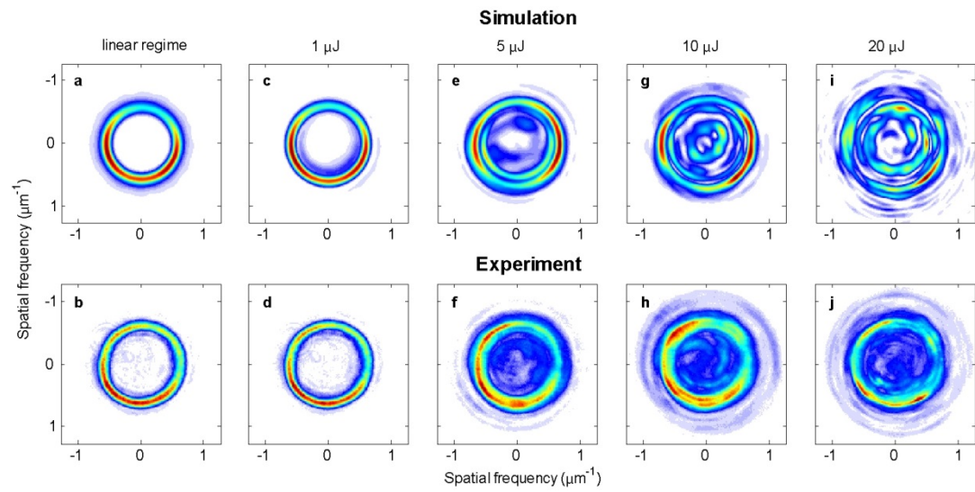
Figure 5. Spatial spectra of linear, stationary (1 μJ), rotating (5 μJ & 10 μJ), and speckle-like (20 μJ) regimes. We compare the far-field fluence distribution for numerical (top) and experimental (bottom row) results at propagation distance z=1 mm. All parameters are identical to those used for figure 4.
