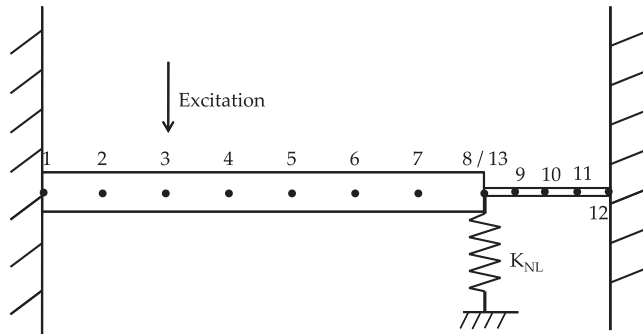
Fig. 1. CostF3 beam.
