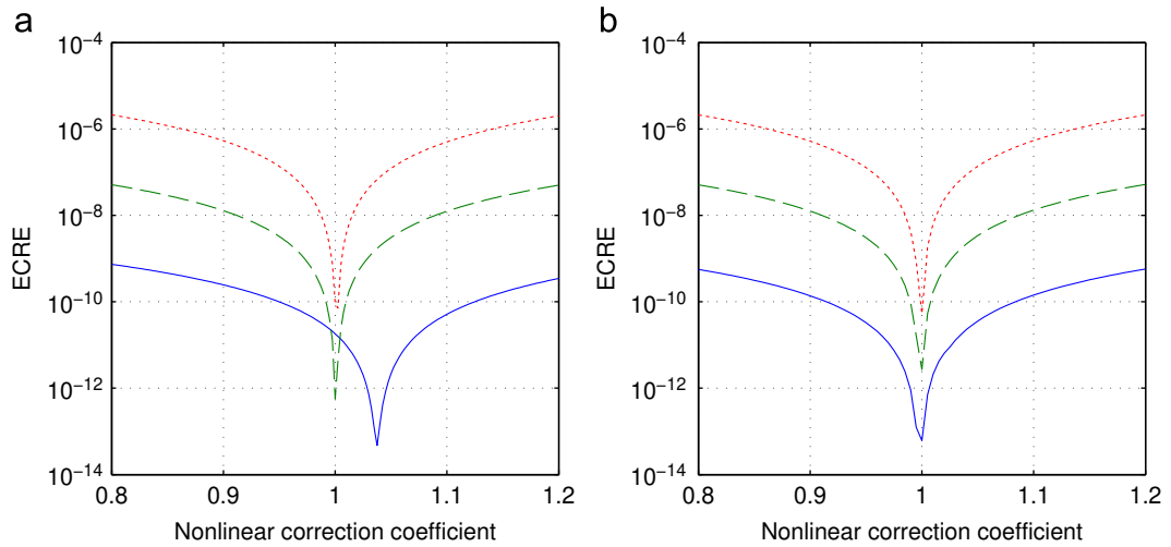
Fig. 10. Four dofs reduced model and three dofs measured: MHB-ECRE results. —, 28 Hz; ---, 30 Hz; - . -, 32 Hz. (a) Fundamental only, (b) fundamental + H3 + H5 + H7.
