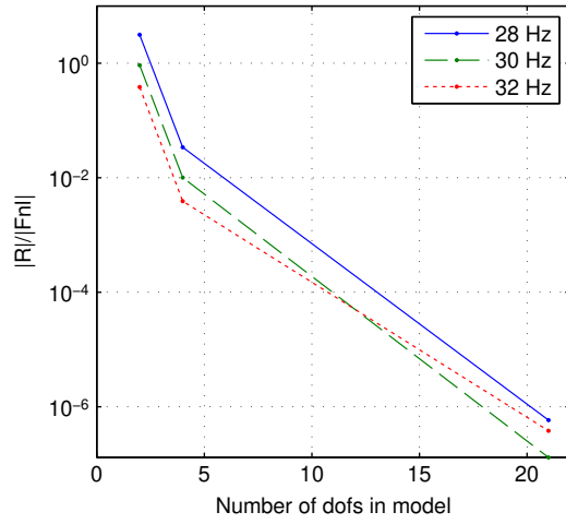
Fig. 8. Influence of model reduction on results accuracy.
