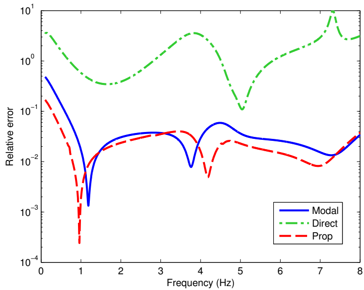
Figure 4: Comparison of relative errors in FRFs - Modal response on perturbed vectors, direct reconstruction, properness enforced reconstruction
