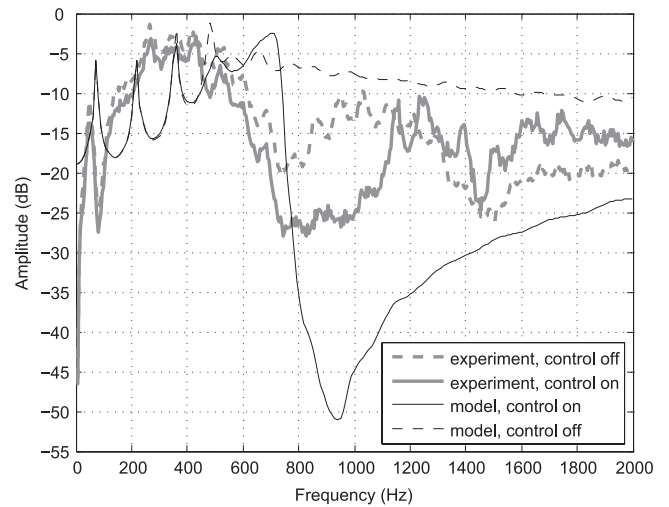
Figure 8. Comparison of transfer functions obtained numerically and experimentally.
