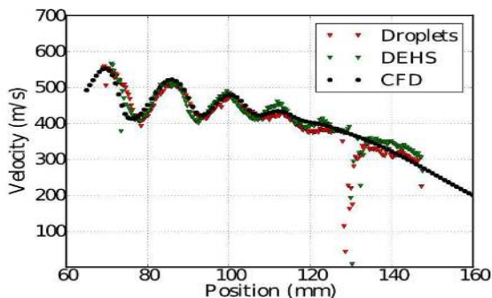
Fig. 5: Evolution of the axial velocity in the mixing tube (with induced flow; P_1 = 4 bar)
