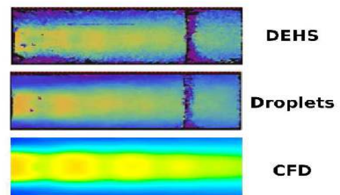
Fig. 6: Comparison of velocity fields (with induced flow; P_1 = 4 bar)
