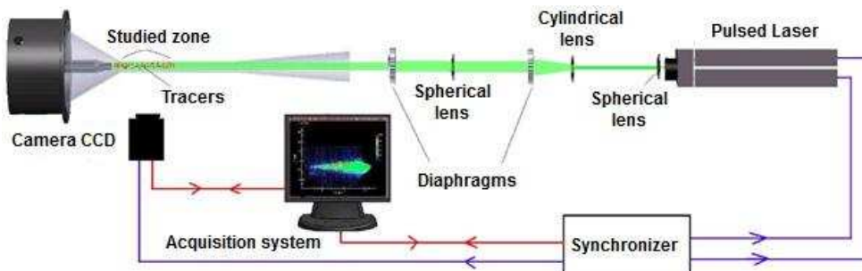
Fig. 2: PIV experimental arrangement
