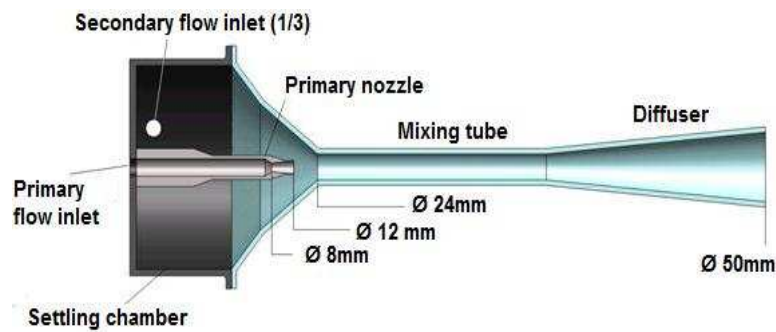
Fig. 1: Ejector configuration
