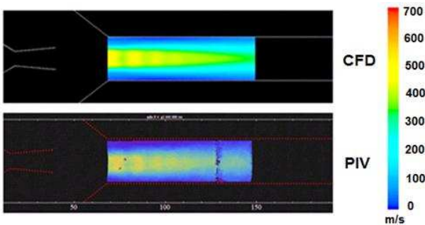
Fig. 3: Comparison of PIV and CFD velocity fields for primary pressure P_1 = 4 bar
