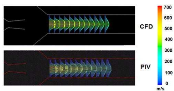
Fig. 4: Comparison of PIV and CFD vectors for primary pressure P_1 = 4 bar
