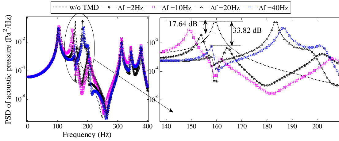
Fig. 9: PSD of acoustic pressure for narrowband and broadband control, \mu=2\% , \omega_2 = 159.52 Hz
