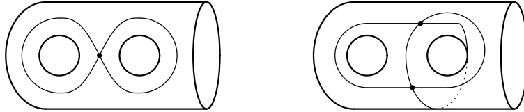
FIGURE 1. Closed curves \gamma such that t_\gamma \notin \mathcal{M}
