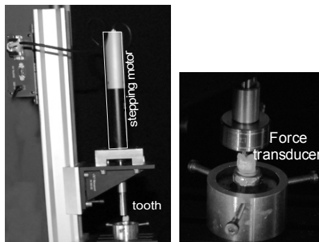
Fig. 2. Compression test mechanical set-up and dedicated molded lower jaw
