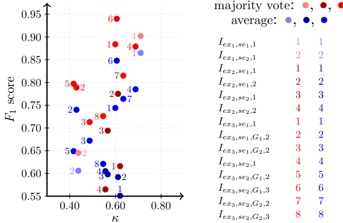
Fig. 4. Overall F_1 scores in relation to Fleiss’ \kappa for inter-annotator agreement (ROI delineation). Shown are the average (blue) and majority vote (red) for different images. Color intensities refer to different experiments. The ids 1–8 are only used to label the dots.
