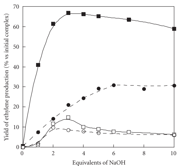
FIGURE 4: Ethylene production by complex 1 (1 mM) in the presence of 10 equivalents of \text{H}_2\text{O}_2 as a function of NaOH added in water (---●---) or in methanol (—■—) and by a mixture of (\text{CuClO}_4 \cdot 6\text{H}_2\text{O} + \text{ACC}) either in water (---○---) or in methanol (—□—).
