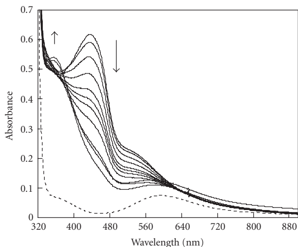
FIGURE 7: UV-visible spectra of 1mM solution of 1 in MeOH with 1 equivalents of NaOH at -20^\circ C : (- - -) initial complex (—) decay of the brown intermediate versus time after addition of 10 equivalents H_2O_2 .
