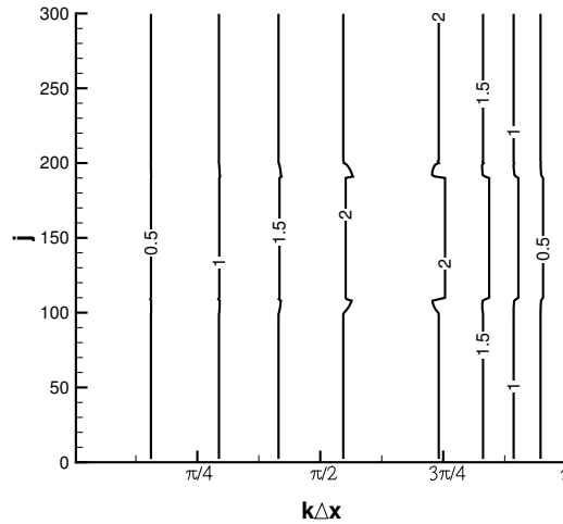
Figure 10: Isocontours of the dispersion \phi_j for the AION scheme and 1 \leq j \leq N at CFL=0.1
