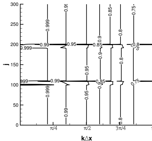
Figure 2: Isocontours of the dissipation coefficient \mu_j for the HCS1 scheme at CFL=0.1
