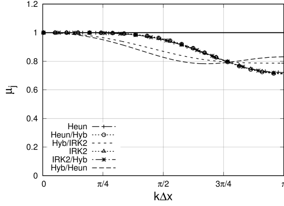
Figure 4: Dissipation \mu_j of the scheme HCS1 for all kinds of cells at CFL=0.1
