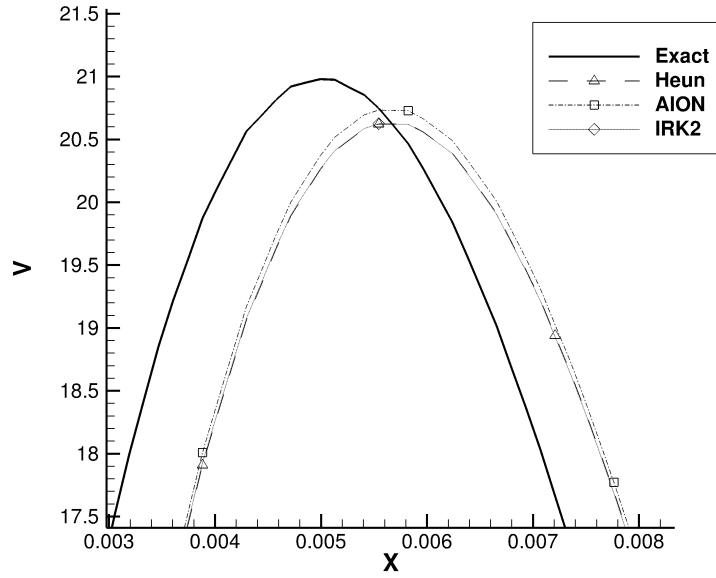
Figure 40: Zoom on the velocity field (CFL=0.1)
