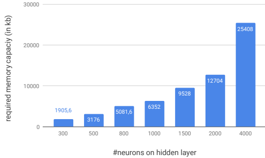
Figure 7: Required memory capacity for a 3 layers classifier with respect to the number of neurons in the hidden layer. Synaptic weights are coded on 1 Byte each. The network has 784 input neurons, and 10 output neurons (typical ANN for testing on MNIST database).
