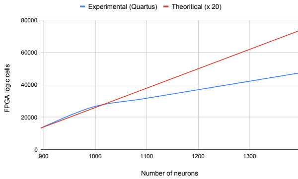
Figure 26: FPA theoretical versus experimental FPGA occupation results with respect to the number of neurons.
