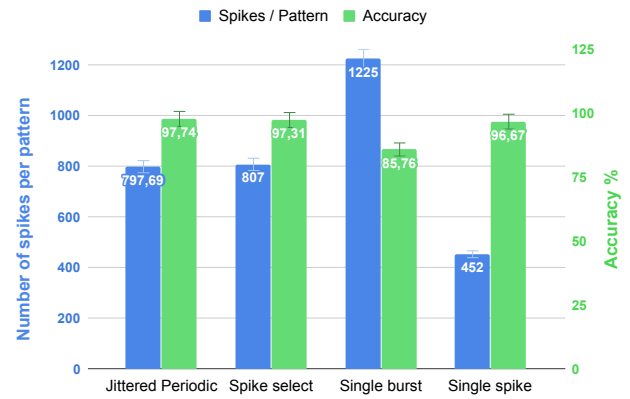
Figure 4: Information coding method impacts the accuracy and the number of spikes processed by the SNN in average for a pattern. The histogram represents results obtained for the 784-300-10 SNN topology using the MNIST test data.
