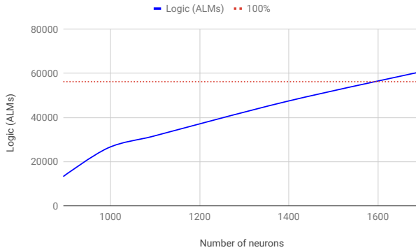
Figure 23: FPA architecture: FPGA logic (ALM) utilization versus the SNN number of neurons; Different SNN topologies are used, see table 8.
