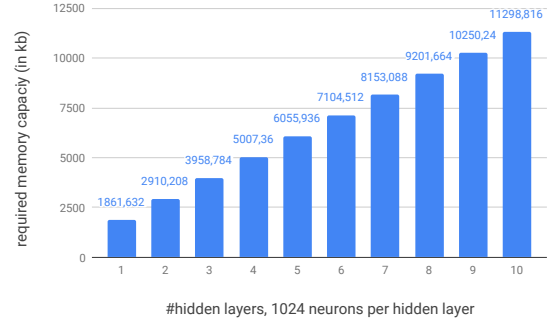
Figure 8: Required memory capacity for a n-layer-classifier, 1024 neurons per hidden layer, with respect to the number of hidden layers. Note that, 1 Byte is used to encode 1 weight and there are 784 input and 10 output neurons.
