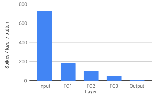
Figure 13: Average number of spikes generated for one MNIST pattern for each layer in the "784-300-300-10" SNN
