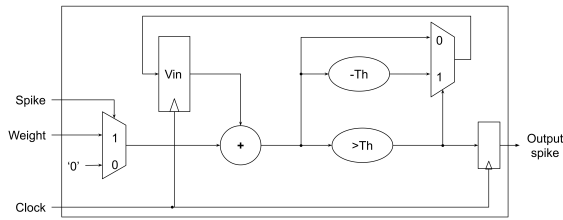
Figure 14: IF neuron module internal structure
