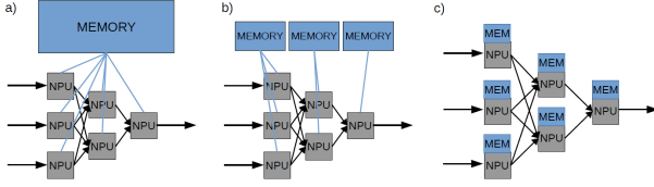
Figure 10: Representation of all memory organizations for fully-parallel architectures: a) centralized memory unit, b) layer-shared memory units, c) fully-distributed memory units
