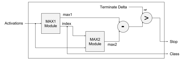
Figure 15: Schematic diagram of the Terminate Delta module
