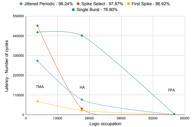
Figure 27: Tradeoff between logic occupation and latency of the hardware architectures according to the different information coding methods. The graph corresponds to FPGA logic occupation in tables 8, 9 and 10) and latency estimation in table 11, which are the data recorded for the SNN of "784-300-300-300-10" topology. The obtained recognition rates on MNIST test dataset with the different methods are indicated in the legend of the figure.
