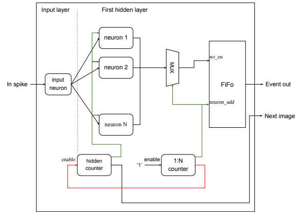
Figure 18: Neural Core simplified schematic diagram. The input neuron forwards input spikes, spike by spike, to the 1 st hidden layer neurons. The 1 st hidden counter is indicating to that hidden neurons the address of the input spike in order to retrieve their appropriate weights. Another counter (1:N) is controlling a MUX component to store the 1 st hidden layer's spikes in a FiFo memory.
