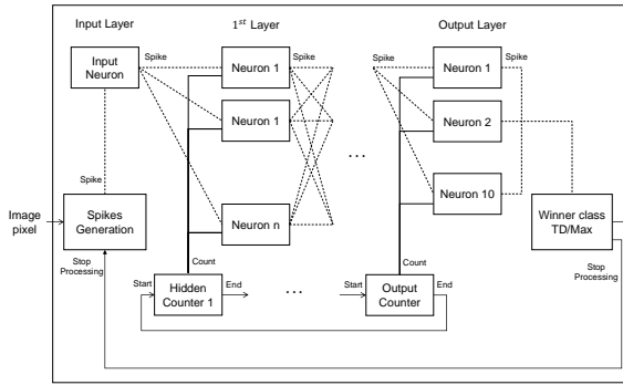
Figure 20: FPA simplified schematic diagram. In this architecture, from the 1 st layer to the output layer all neurons are implemented in hardware. Counters connected in series are coordinating the processing of the different network spikes in a coherent way.
