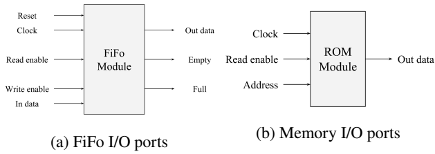
Figure 17: FiFo and memory I/O port blocks
