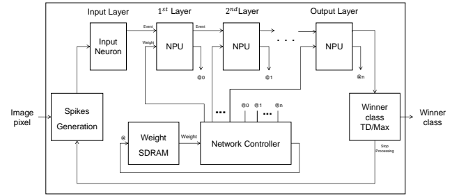
Figure 21: TMA simplified schematic diagram. Here, the input neuron module forwards input spikes to NPUs connected in series, each NPU represents a distinct layer, that execute the SNN neurons to finally using the winner class selection module output the SNN's class.
