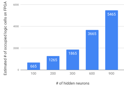
Figure 9: Theoretical values for FPGA occupation against hidden layer size. 784 input and 10 output neurons.
