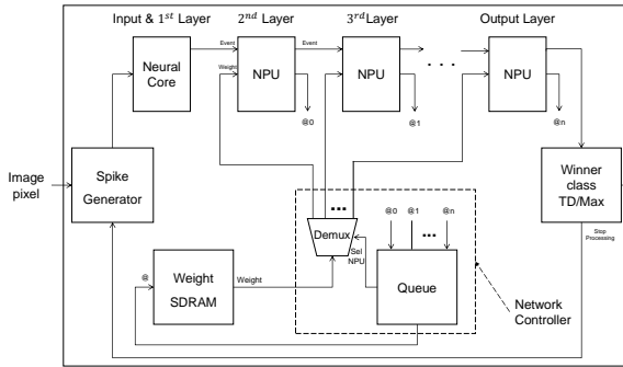
Figure 22: Hybrid architecture simplified schematic diagram. The input and the 1 st layers are implemented using a Neural Core and NPUs are used for the remaining layers (one NPU per layer). The output layer spikes are fed to the winner class selection module for classification. A Network Controller is used to manage and connect the NPUs to an SDRAM holding their logical weights.
