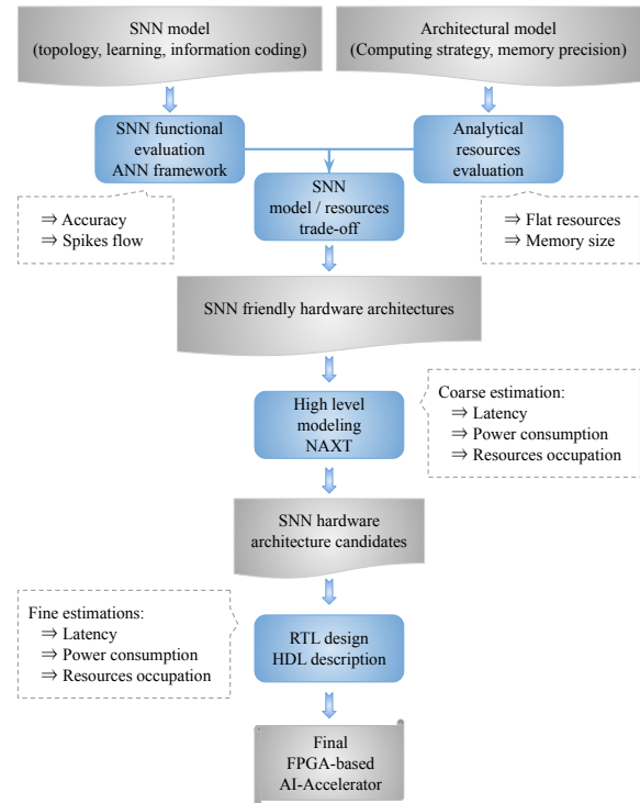
Figure 6: Design Flow Diagram. First stage: Perform a functional evaluation of different SNN models using an ANN framework (N2D2). Simultaneously, using an analytic model evaluate the cost (memory size and flat resources) of some architectural models. Then, make a model / resources trade-off to select some SNN friendly hardware architectures; Second stage: High-level simulation of the chosen topology with different architectural choices, to select the architectural paradigm for the last stage; Third stage: Develop RTL designs of the SNN hardware architecture candidates to have finer cost estimations. Then, based on these results select one architecture as the final FPGA-based AI-Accelerator.
