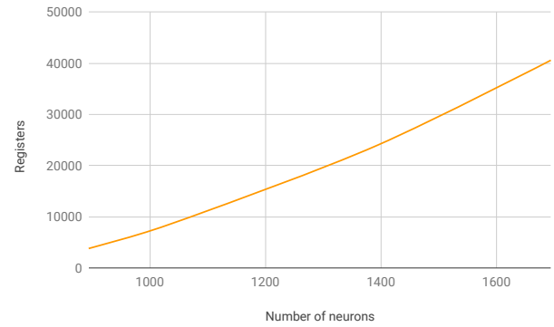
Figure 24: FPA architecture: FPGA registers occupation versus the SNN number of neurons; Different SNN topologies are used, see table 8.
