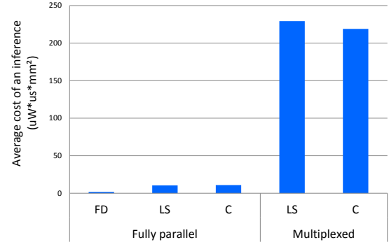
Figure 12: Qualitative cost function for a 804 neurons hardware SNN for the different architectures available in NAXT
