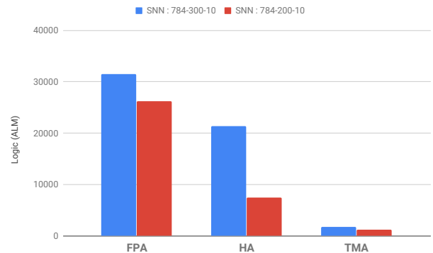
Figure 25: Logic occupation of two SNN topologies comparing the three architectures (FPA, TMA and HA)
