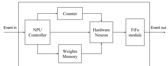
Figure 19: Neural Processing Unit simplified block diagram. When there is an input event to process by the NPU: first, the hardware neuron is enabled by the NPU controller to retrieve the address of the logical neuron it represents from the counter and the corresponding weights from the memory block. Second, do its computation, and whenever it fires, the output spikes is stored in a FiFo as an event.
