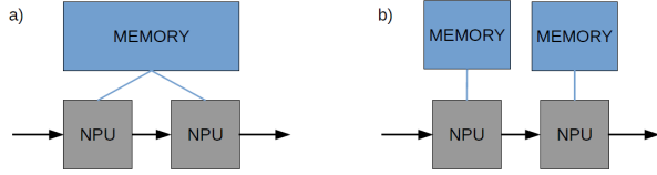
Figure 11: Representation of all memory organizations for TMA: a) centralized memory unit, b) layer-shared/fully-distributed memory units
