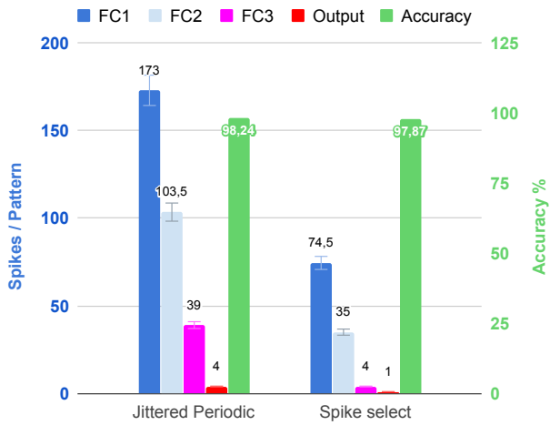
Figure 5: Spike Select versus Jittered Periodic in terms of accuracy and number of spikes generated for a pattern in SNN deeper layers. The histogram represents results obtained for the 784-300-300-300-10 SNN topology using the test data of MNIST (cf table 4).
