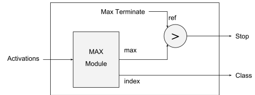
Figure 16: Schematic diagram of the Max Terminate module
