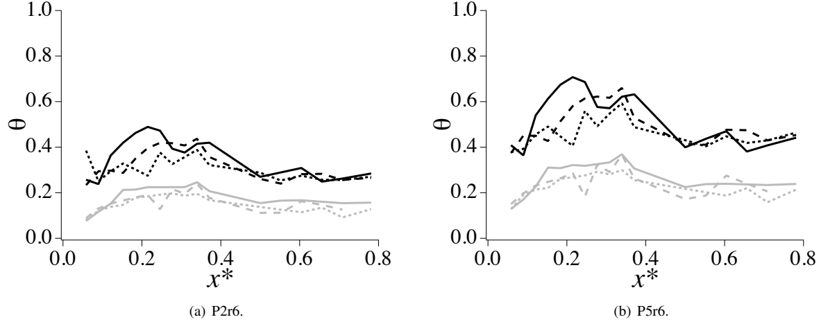
Fig. 6 Reduced temperature profiles on the hot side (black) and cold side (grey), versus longitudinal coordinate for cases at mixture ratio r = 6 . Location A (— and —); location B (----- and -----); location C (---- and ----) in Fig. 1(b).
