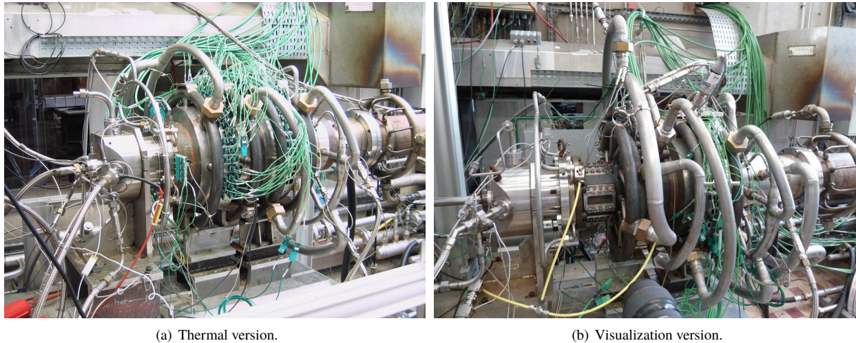
Fig. 2 Photograph of the Bhp-HrM experiment operated at ONERA on the Mascotte test bench.
