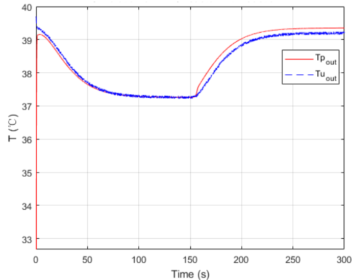
Figure 14. Simulated temperature profiles for experiment 1 (reaction was introduced at 150 s).
