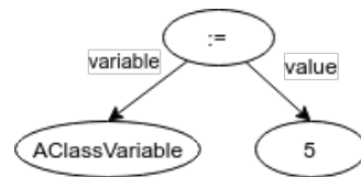
Figure 7. Pharo AST for the expression: AClassVariable := 5. It is represented by an AssignmentNode assigning to the variable AClassVariable the literal value 5.
