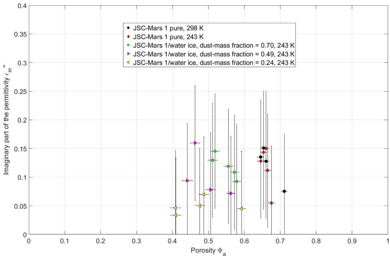
Fig. 6. Mean of the imaginary part of the permittivity ( \epsilon_m'' ) calculated over the relevant frequency range as a function of the porosity ( \phi_a ) for pure JSC Mars-1 samples measured at 298 K and 243 K, and for mixtures consisting of JSC Mars-1 and pure water ice with dust mass fractions equal to 0.70, 0.49 and 0.24. The error bars represent the maximum experimental uncertainty.
